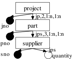
Fig. 1(b). ORA-SS schema of document in Fig. 1(a)
