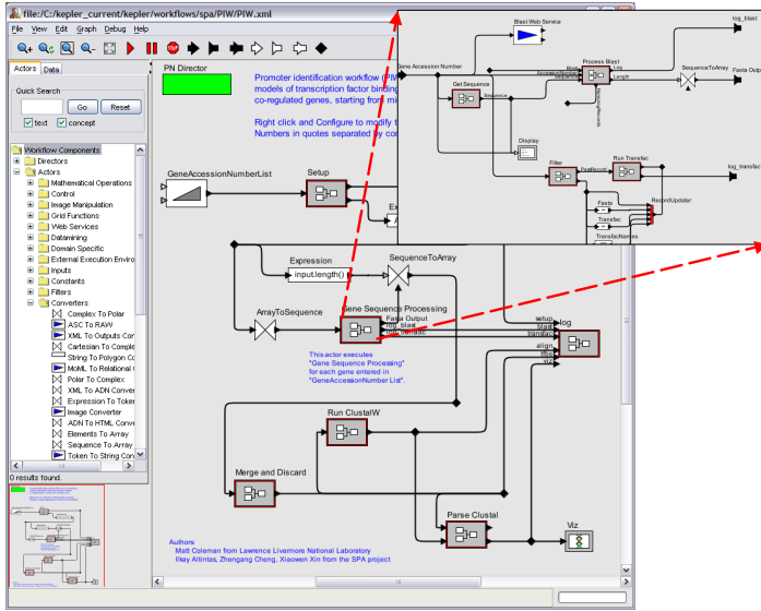
Fig. 1. A bioinformatics workflow in KEPLER: the composite actor (center) contains a nested subworkflow (upper right); workflow steps include remote service invocation and data transformation; and the execution model is enforced by a director (green box)
