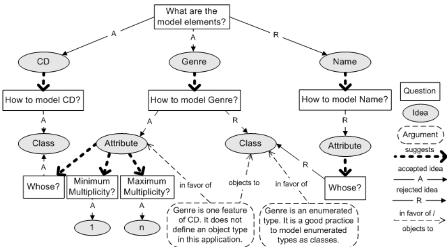
Fig. 3. A portion of a DR representation regarding “ Genre ” in the motivating example (Fig. 1)
