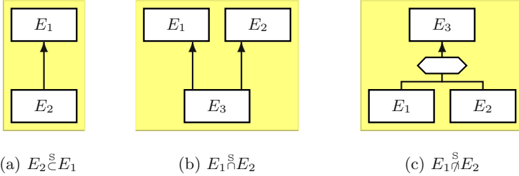
Fig. 3. Partial Integrated Schemas: ER Entity Subsumption, Intersection, Disjointness
