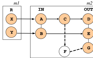
Fig. 3. A modular system graph containing two modules
