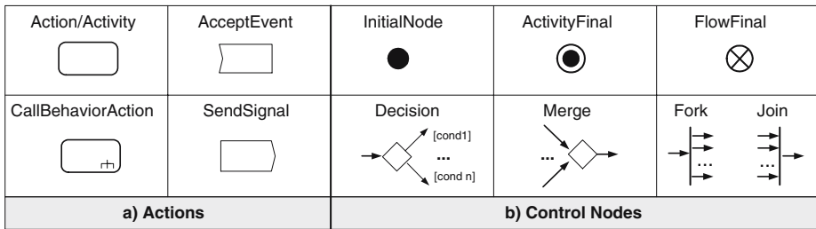
Fig. 1. UML 2.0 AD, Main Symbols
