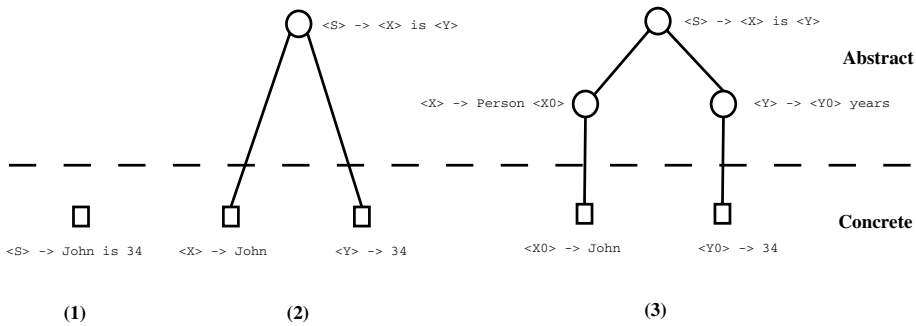
Fig. 2. Parsing levels
