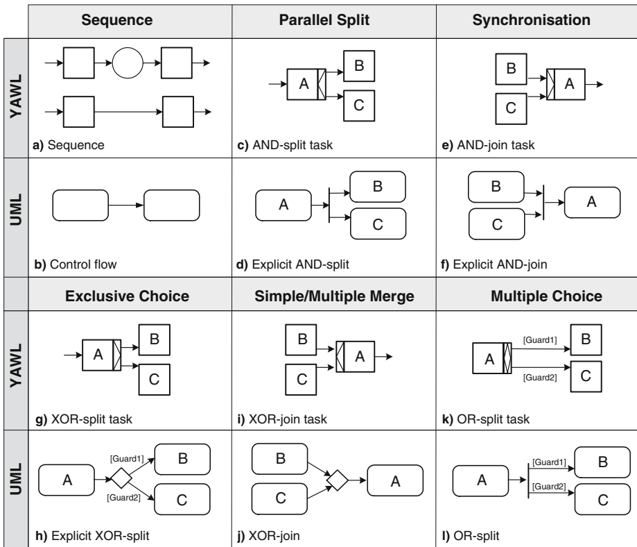
Fig. 2. Basic Control-flow Constructs in UML AD and in YAWL
