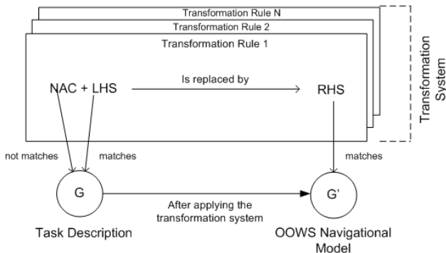
Fig. 6. A transformation system
