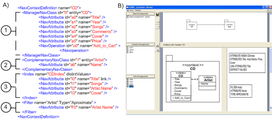
Fig. 13. An OOWS XML specification and the OOWS case tool
