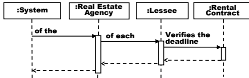
Fig. 2. An example of an Interaction Fragment
