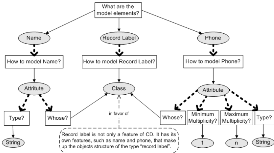
Fig. 6. Example of DR about the Record Label information item
