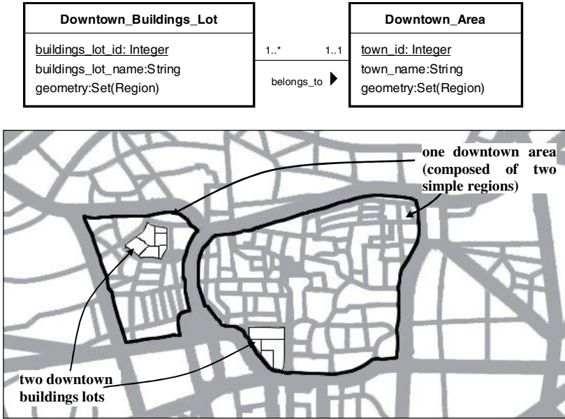
Fig. 4. “Downtown building lot” example
