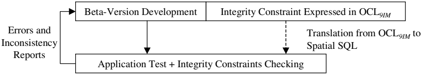
Fig. 7. Example of development process with OCL_{9IM}
