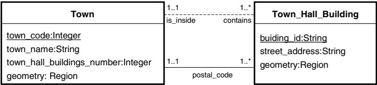
Fig. 1. “Town hall building” example
