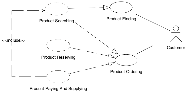
Fig. 1. The TLOOF diagram of an ordering system
